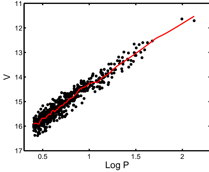
Figure 5: An illustrative loess regression on the OGLE PL data. The window width is 0.05, i.e. 5% of the range of \text{log } P .
