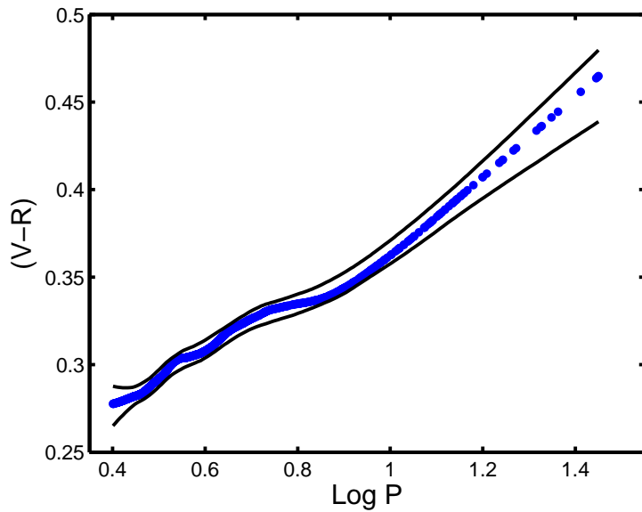
Figure 19: A loess regression function fitted to the \log P – (V - R) data from the MACHO observations. The solid lines are the 95% confidence envelopes, obtained by bootstrapping.
